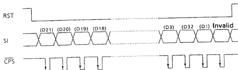
Fig. 34 M56760 PLL DATA OUTPUT
