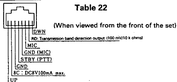
Fig. 43 Microphone Socket (on Front Panel)
